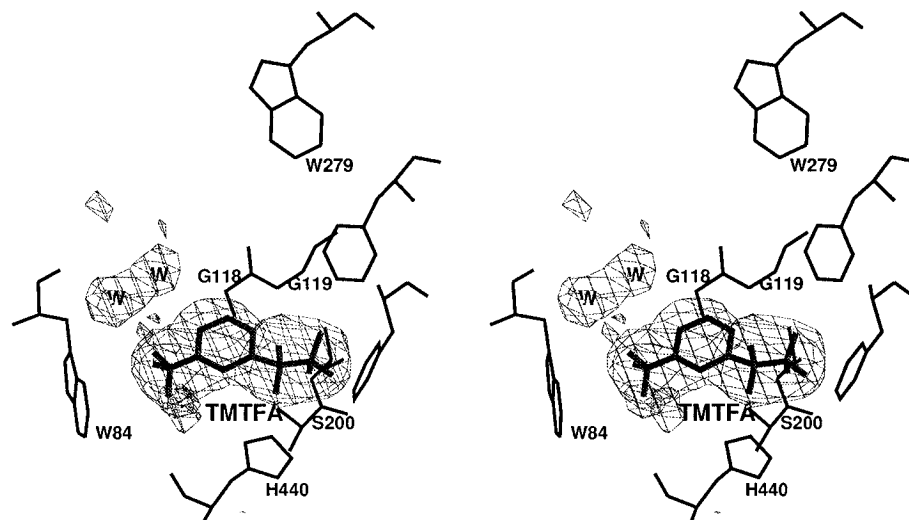
Figure 2. Omit map of the refined structure of the TMTFA–TcAChE complex contoured at 3\sigma and displayed in stereo. The final refined coordinates are superimposed on the electron density map. Electron density interpreted as water molecules is marked by the letter W. The residue that extends behind the electron density of the bound inhibitor is A201.
