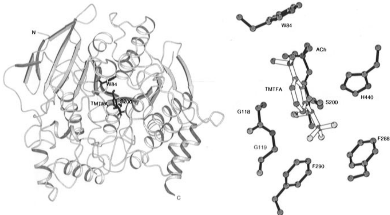
Figure 3. (A, left) Overall conformation of the TMTFA–TcAChE complex. The side chains of S200 of the catalytic triad and of W84, which interacts with the quaternary nitrogen group, are shown together with TMTFA. (B, right) Closeup of the active site of the TMTFA–TcAChE complex, showing the experimentally determined TMTFA (open-face lines) with a superimposed model of ACh docked in the active site (solid lines). 9 Several key residues in the binding pocket are indicated.
